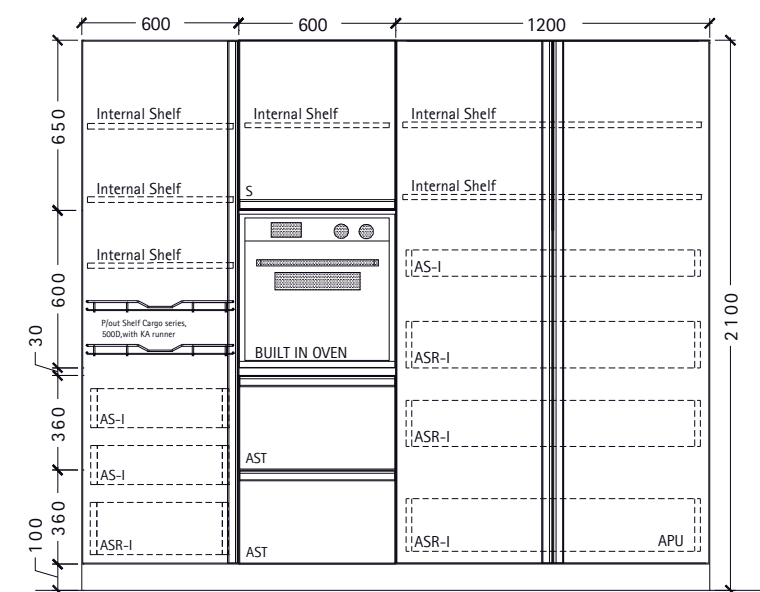
Elevation C
