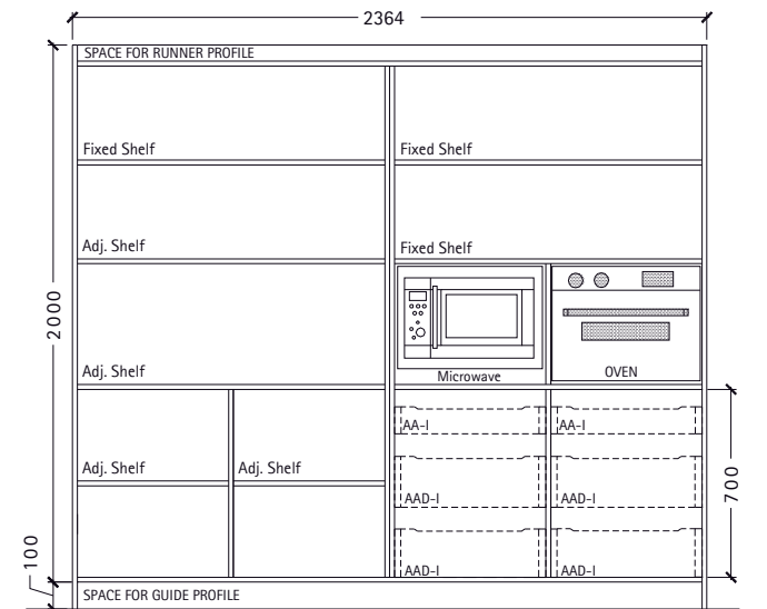
InLine XL- Internal Elevation
