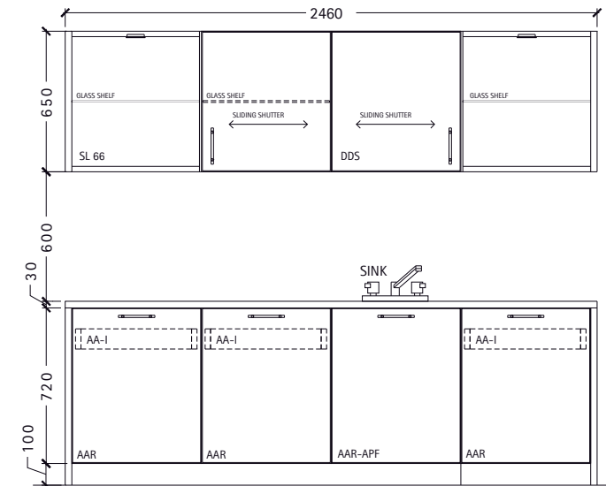
Elevation C
