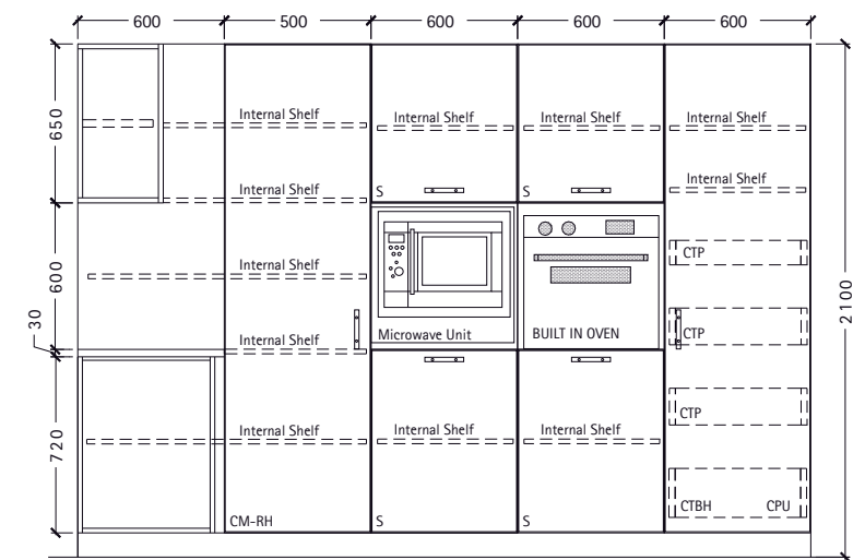
Elevation C
