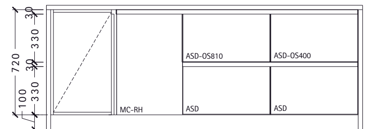
Island Elevation
