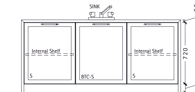
Island Elevation
