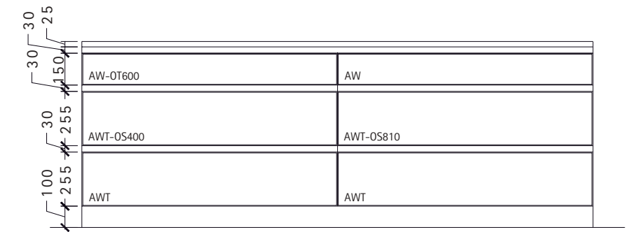
Elevation C
